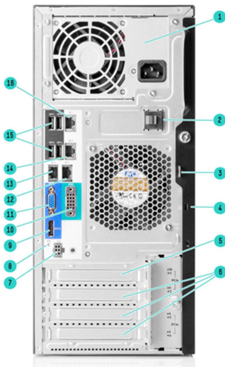
Rear View 4LFF Gen11
